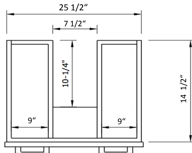
TOP DRAWER
