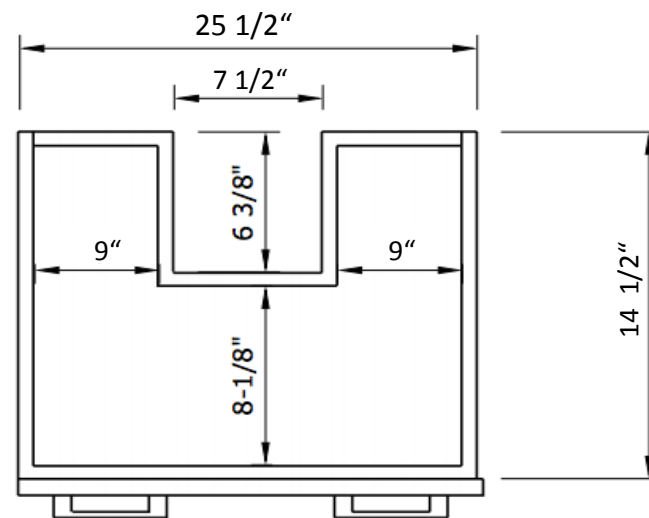
BOTTOM DRAWER
