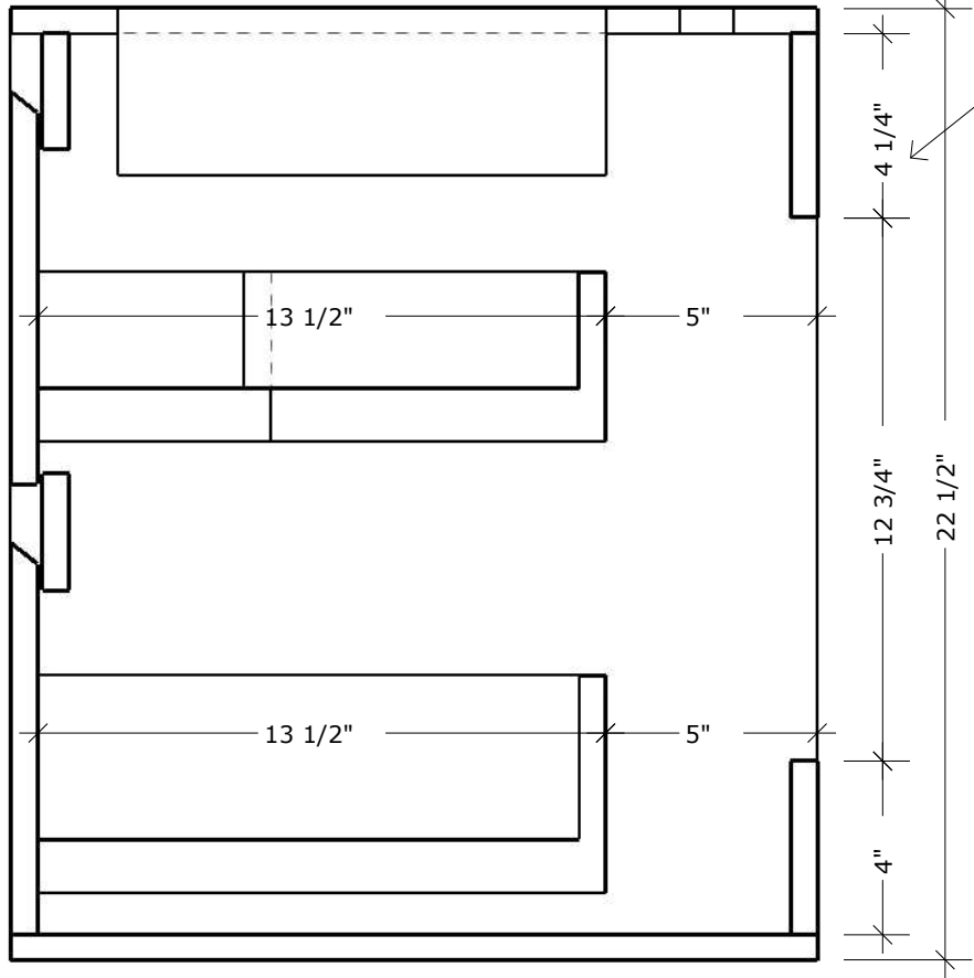
SECTION CUT
