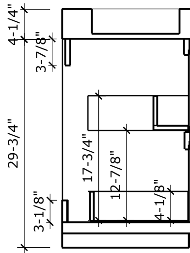
SECTION CUT
