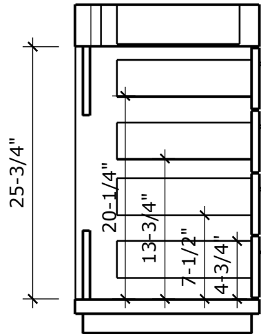
SECTION CUT
